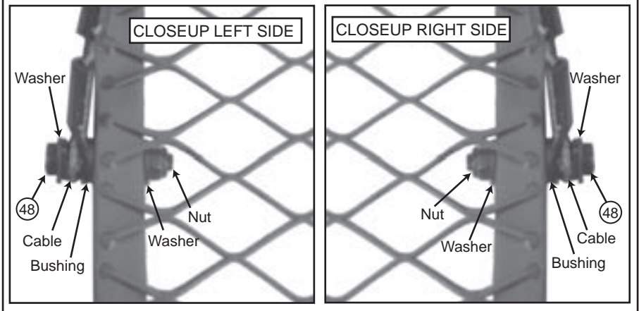
Cable to Platform
