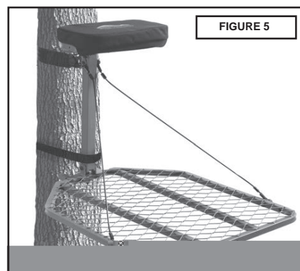
FIGURE 5: ATTACH BUCKLE STRAP TO VERTICAL SUPPORT TO SECURE STAND TO TREE
