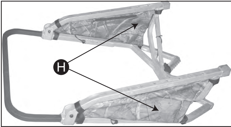
7. Attach Accessory Pouch H to the frame of the seat platform as shown.
