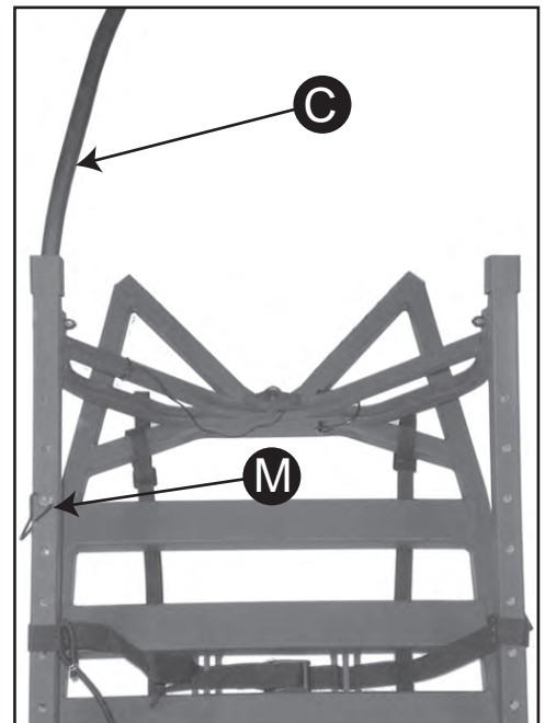
11. Insert one end of Cable C into Foot Platform Rail. Insert 1 - M12 Quickclip M into the rail and through the eyelet on the cable.
