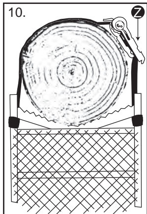
10. Cautiously climb to the top of the treestand. Wrap the strap of the ratchet around the back of the tree and thread it through the ratchet. (See Detailed Ratchet Instructions Below).
