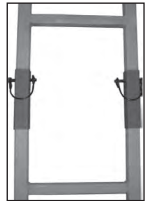
19. Close the quickclip to secure the ladder sections together.
