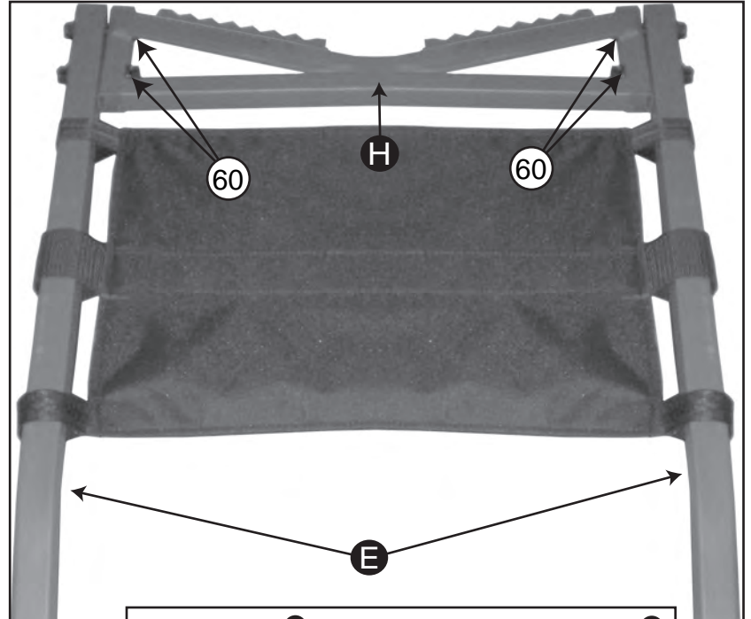
4. Attach V-Bar H between the ends of Handle Rails E using 2- M12x60mm bolts on each side.
