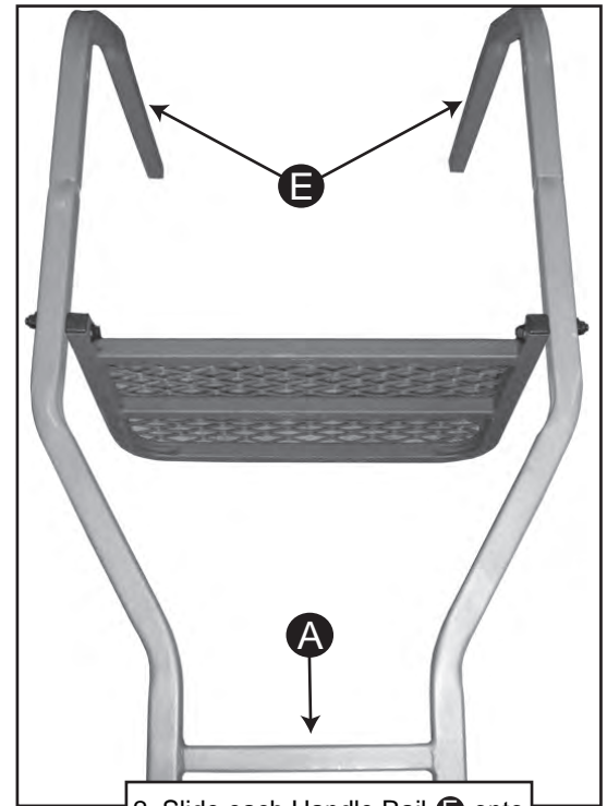
2. Slide each Handle Rail E onto Top Ladder Section A .
