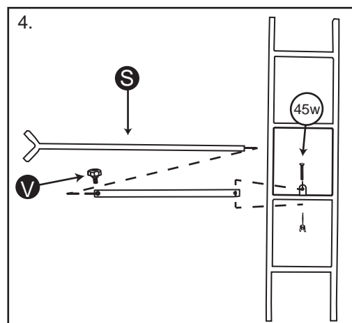
4. Slide the inner part of the Stabilizer Bar into the outer part. Attach Stabilizer Bar S to the second rung of the Middle Ladder Section with 1 - M12x45mm bolt and 1 wingnut .
