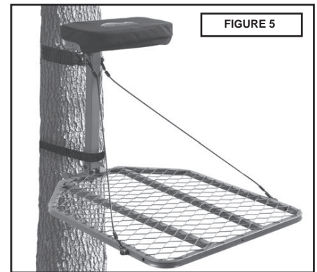
FIGURE 5: ATTACH BUCKLE STRAP TO VERTICAL SUPPORT TO SECURE STAND TO TREE
